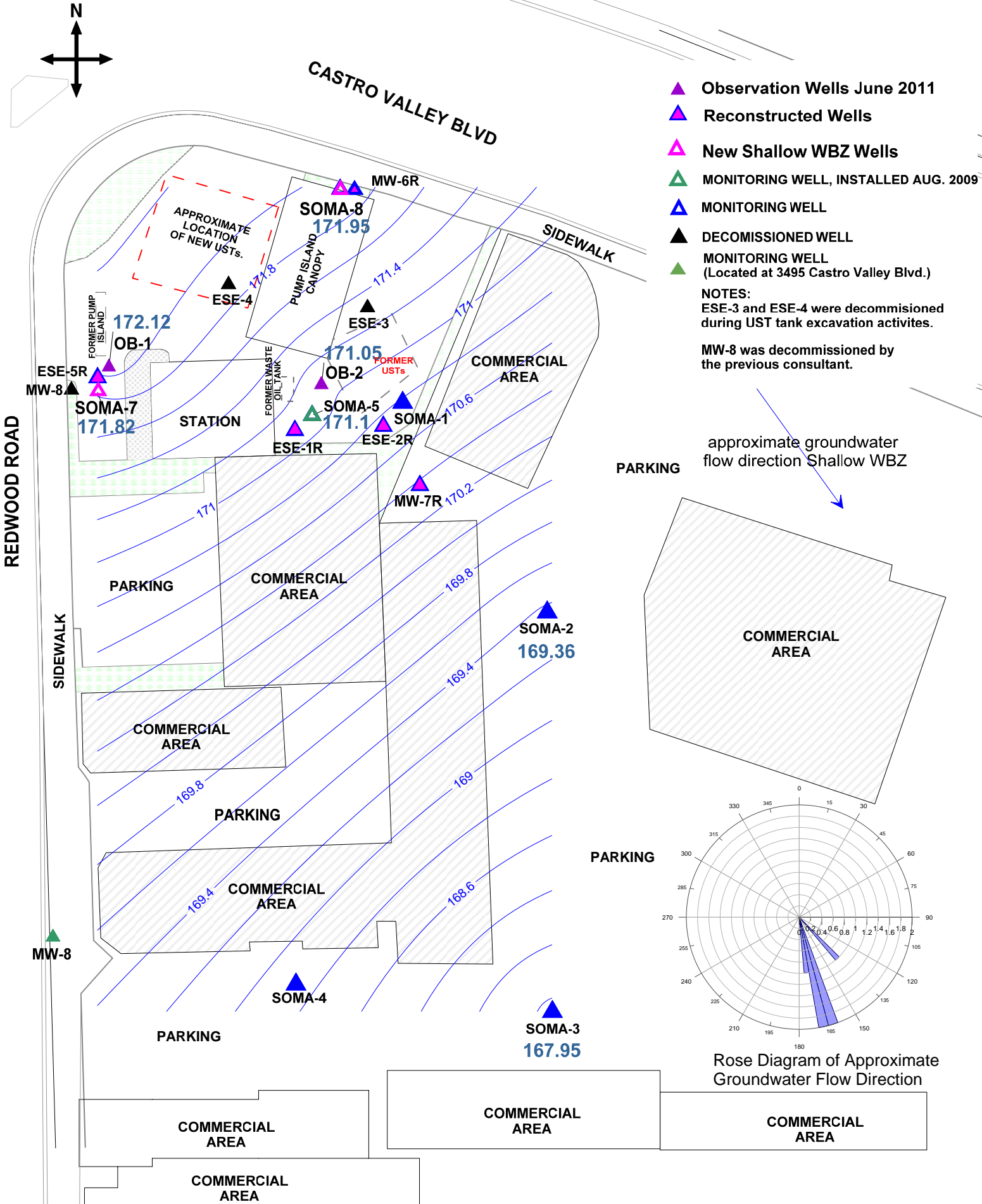
Figure 3: Groundwater Elevation Contour Map for Shallow WBZ Wells in Feet. January 9, 2013
