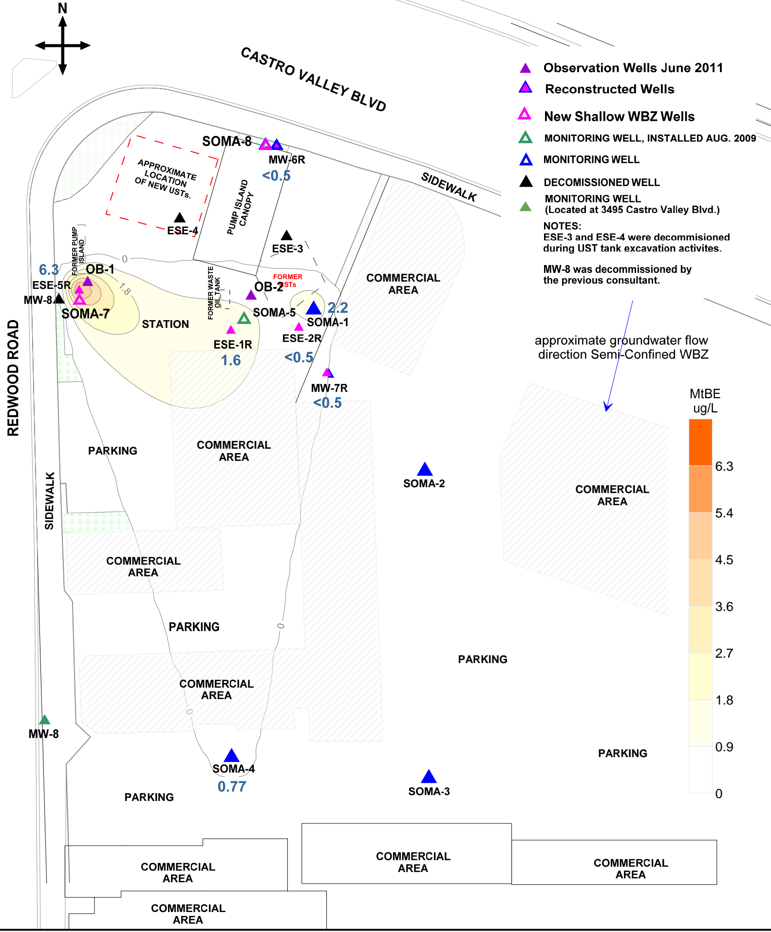
Figure 9: Contour Map of MtBE Concentrations in Semi-Confined WBZ Wells. January 9 and 10, 2013
