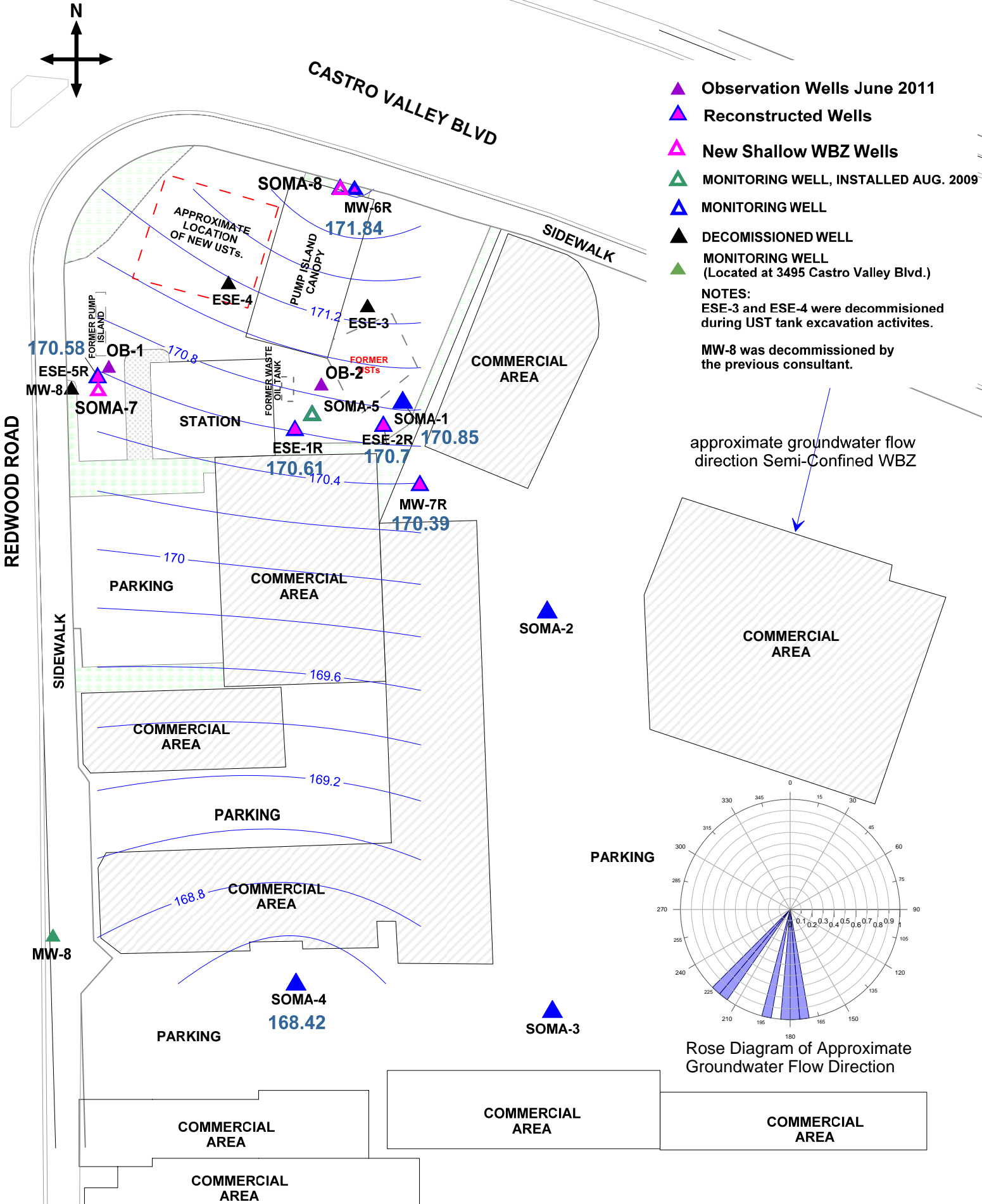
Figure 7: Groundwater Elevation Contour Map for Semi-Confined WBZ Wells in Feet. January 9, 2013
