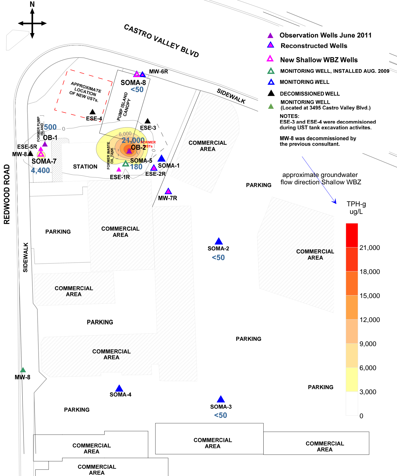
Figure 4: Contour Map of TPH-g Concentrations in Shallow WBZ Wells in Feet. January 9 and 10, 2013
