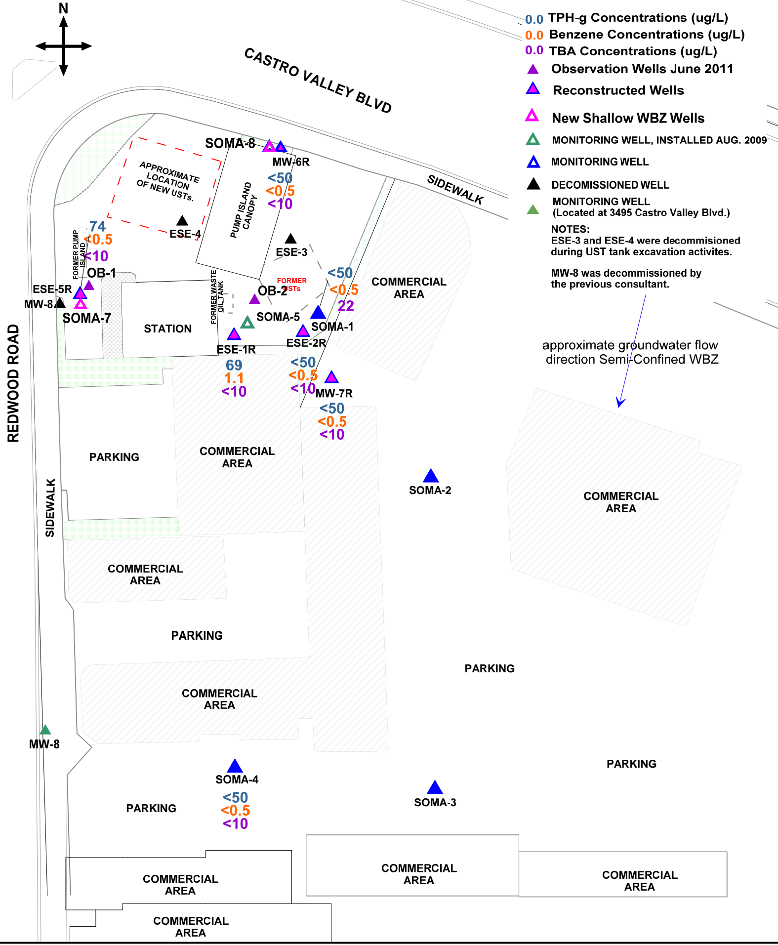
Figure 8: Map of TPH-g, Benzene and TBA Concentrations in Semi-Confined WBZ Wells. January 9 and 10, 2013
