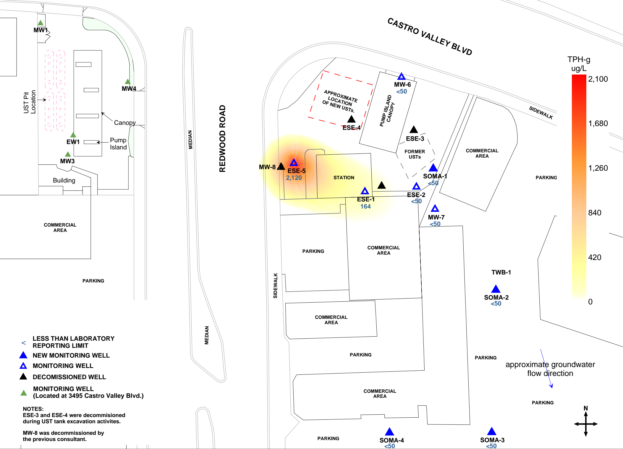
Figure 4: Contour map of TPH-g concentrations in groundwater. October 16, 2007.
