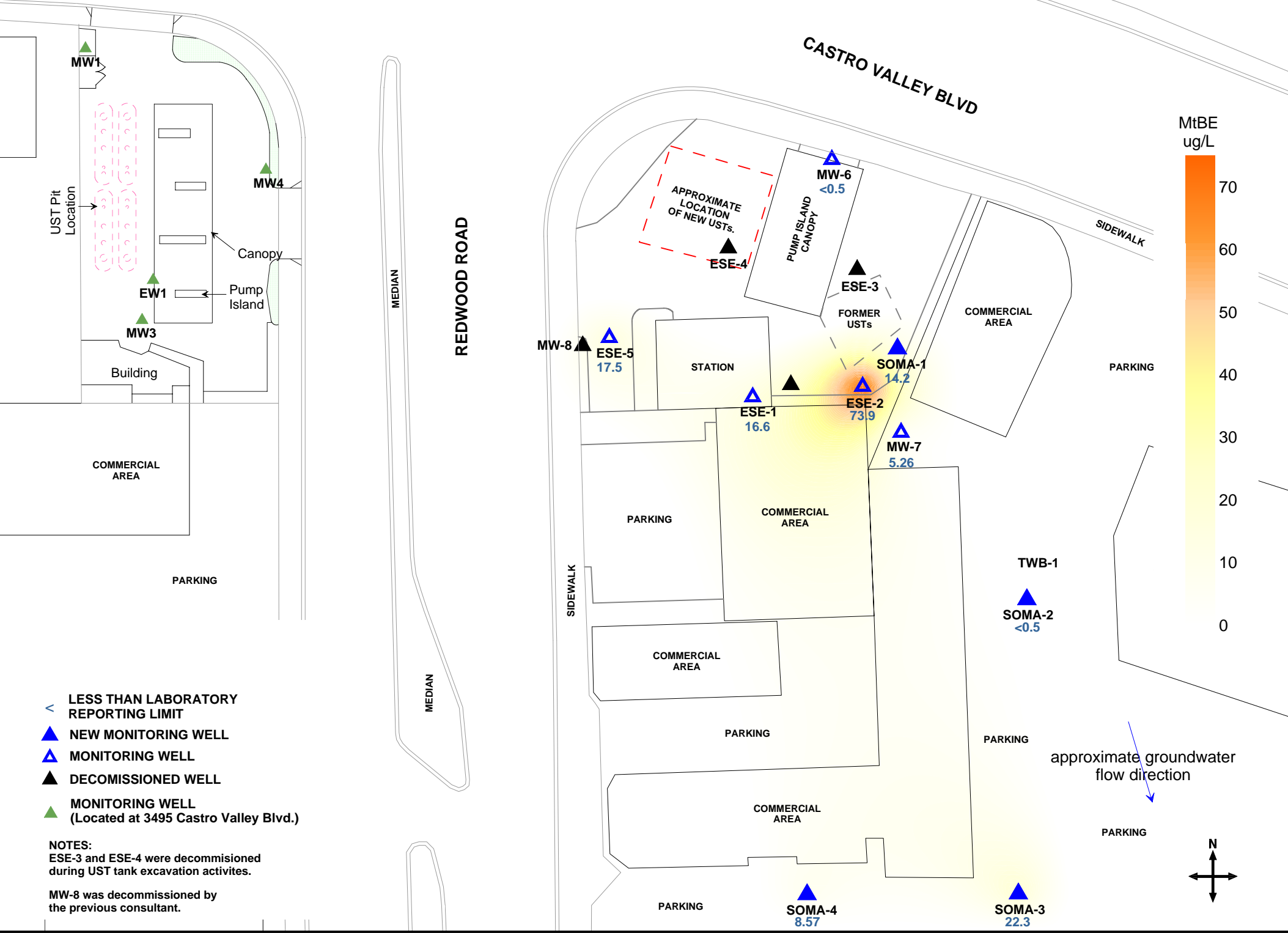
Figure 5: Contour map of MtBE concentrations in groundwater. (EPA Method 8260B). October 16, 2007.
