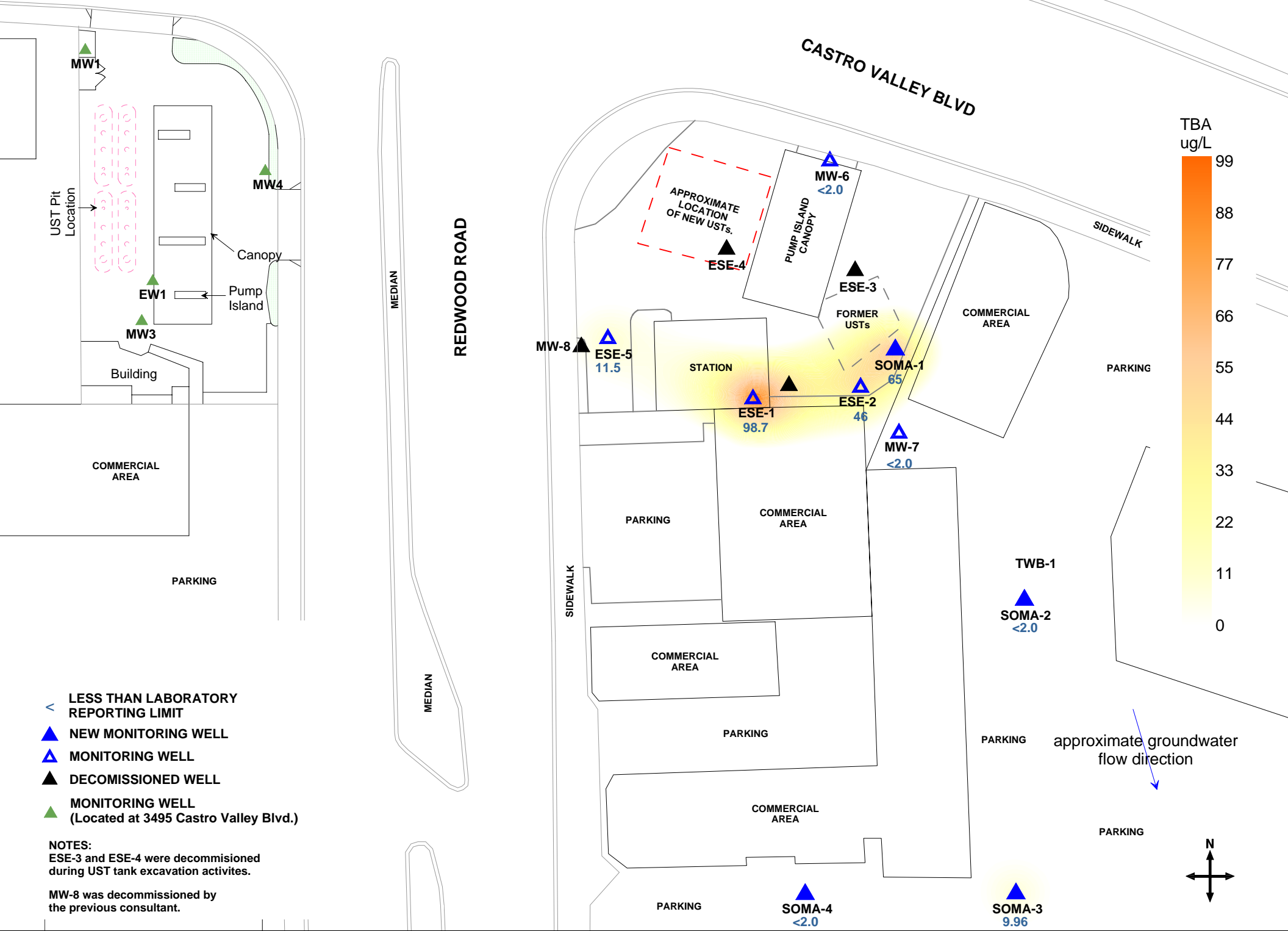
Figure 6: Contour map of TBA concentrations in groundwater. October 16, 2007.
