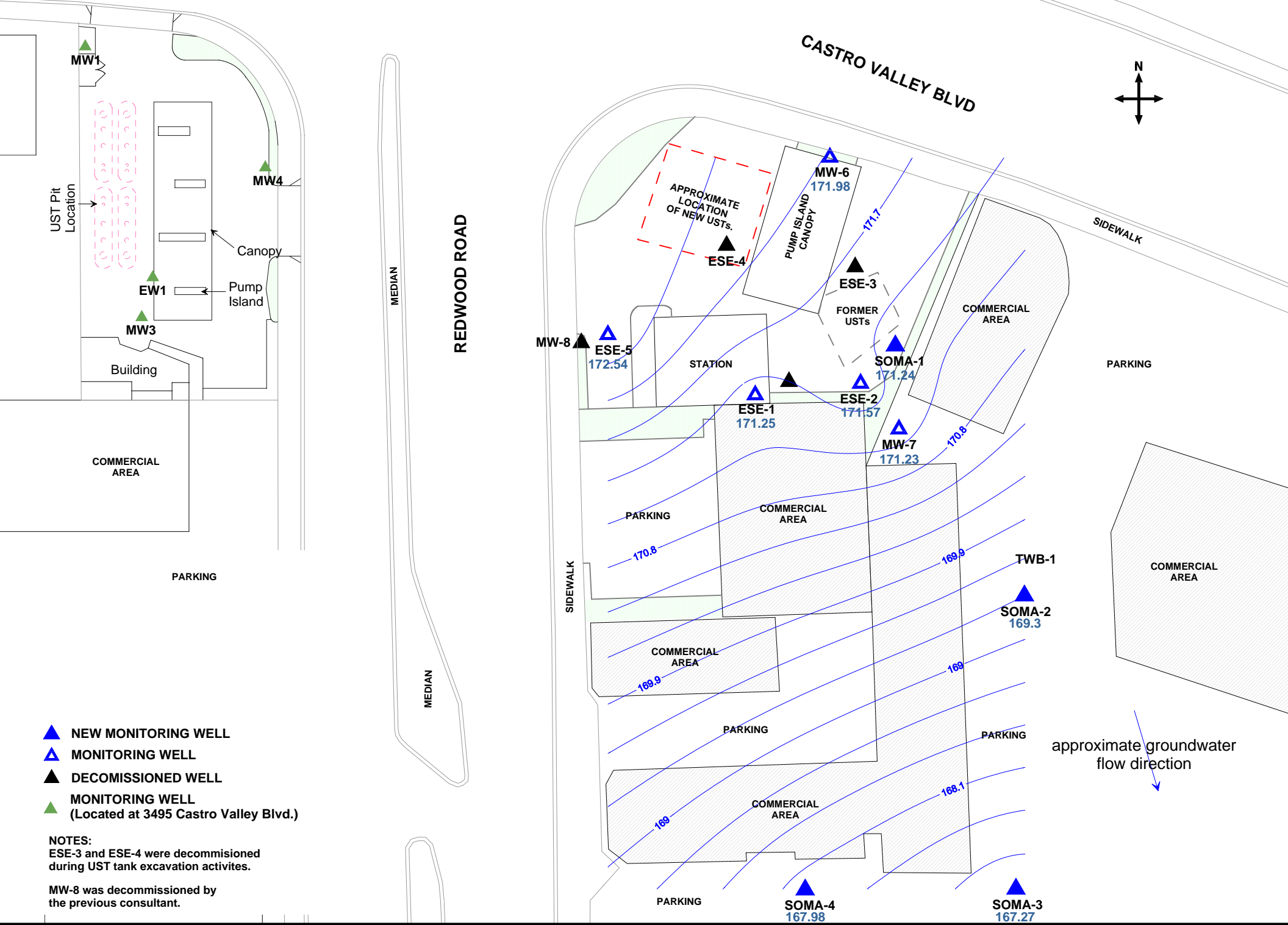
Figure 3: Groundwater elevation contour map in feet. October 16, 2007.
