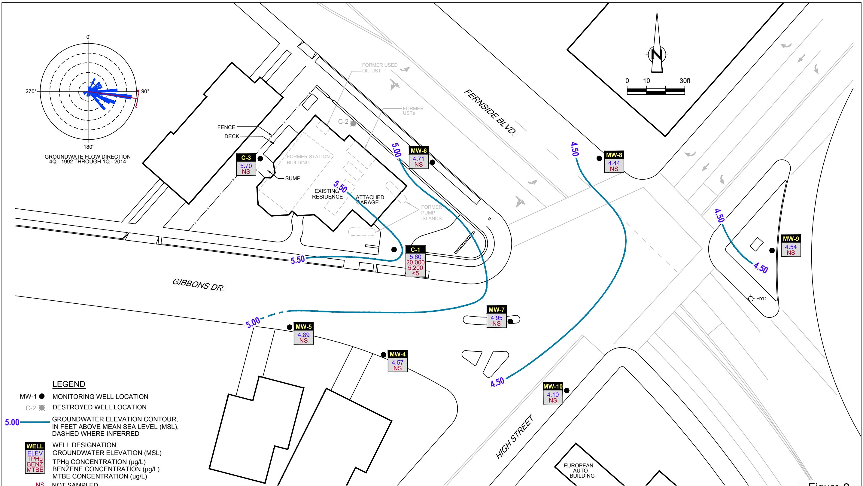
Figure 2 GROUNDWATER ELEVATION AND HYDROCARBON CONCENTRATION MAP FORMER CHEVRON SERVICE STATION 91153 3135 GIBBONS DRIVE (3126 FERNSIDE BLVD) Alameda, California December 30, 2014
