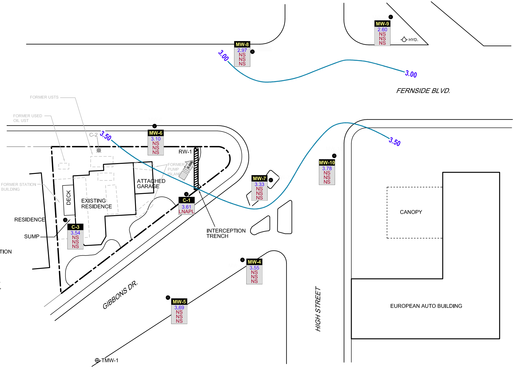
Figure 2 GROUNDWATER ELEVATION AND HYDROCARBON CONCENTRATION MAP FORMER CHEVRON SERVICE STATION 91153 3135 GIBBONS DRIVE (3126 FERNside BLVD) Alameda, California June 28, 2013
