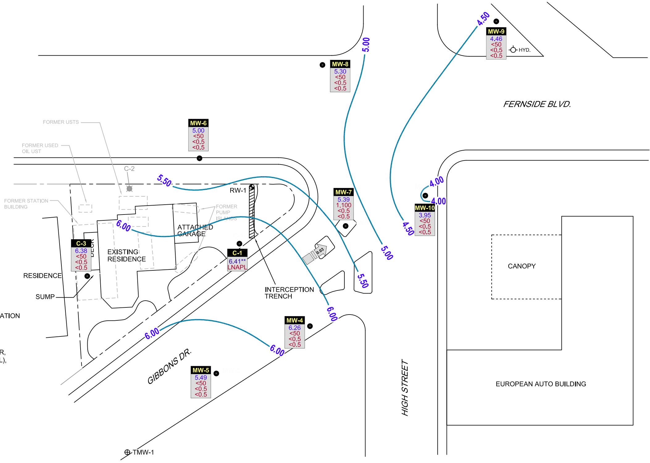
Figure 2 GROUNDWATER ELEVATION AND HYDROCARBON CONCENTRATION MAP FORMER CHEVRON SERVICE STATION 9-1153 3135 GIBBONS DRIVE (3126 FERN SIDE BLVD) Alameda, California March 2, 2011
