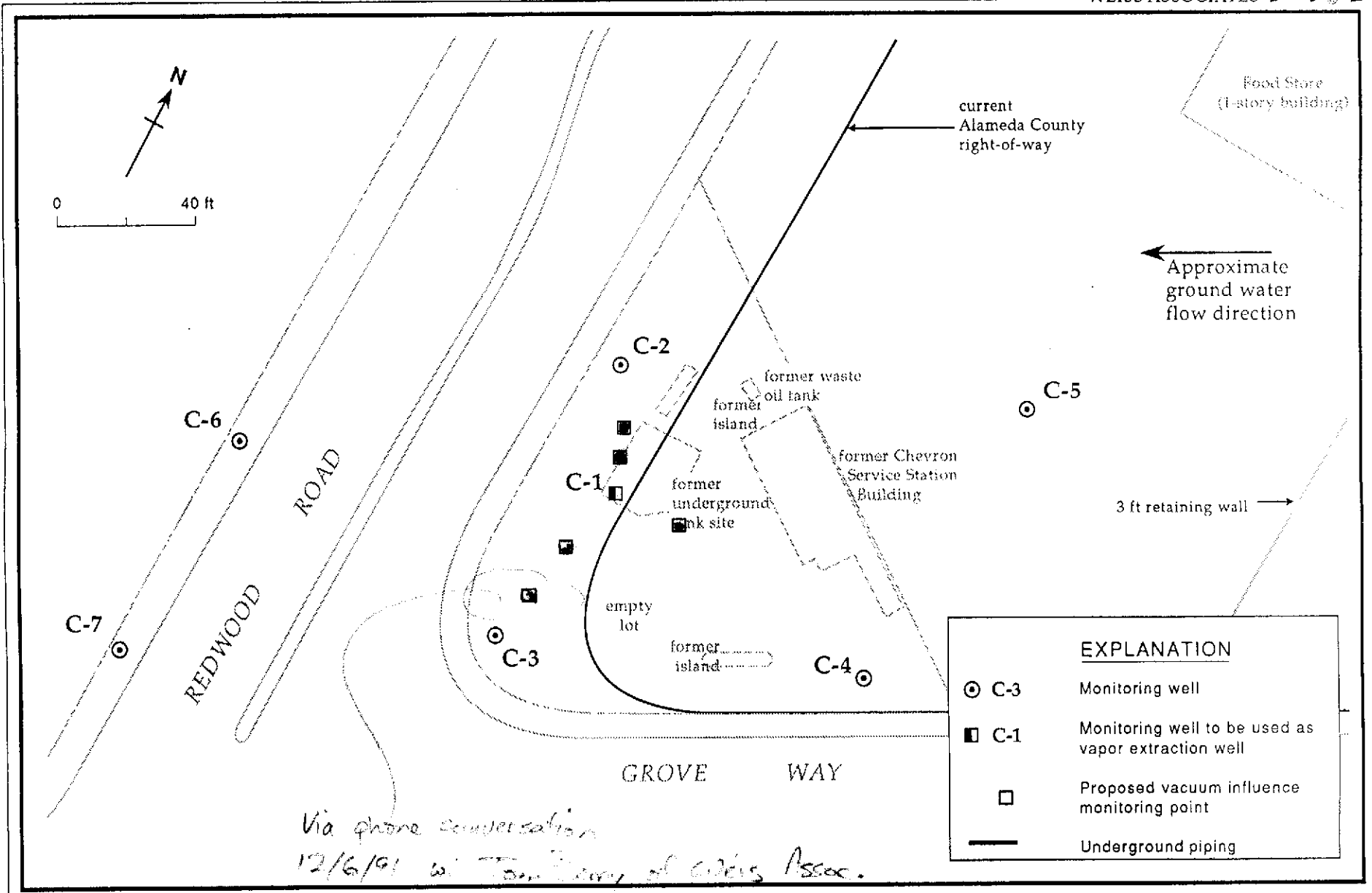
Figure 2. Proposed Extraction and Monitoring Locations for Vapor Extraction Test - Former Chevron Service Station #9-2960, 2416 Grove Way, Castro Valley, California
