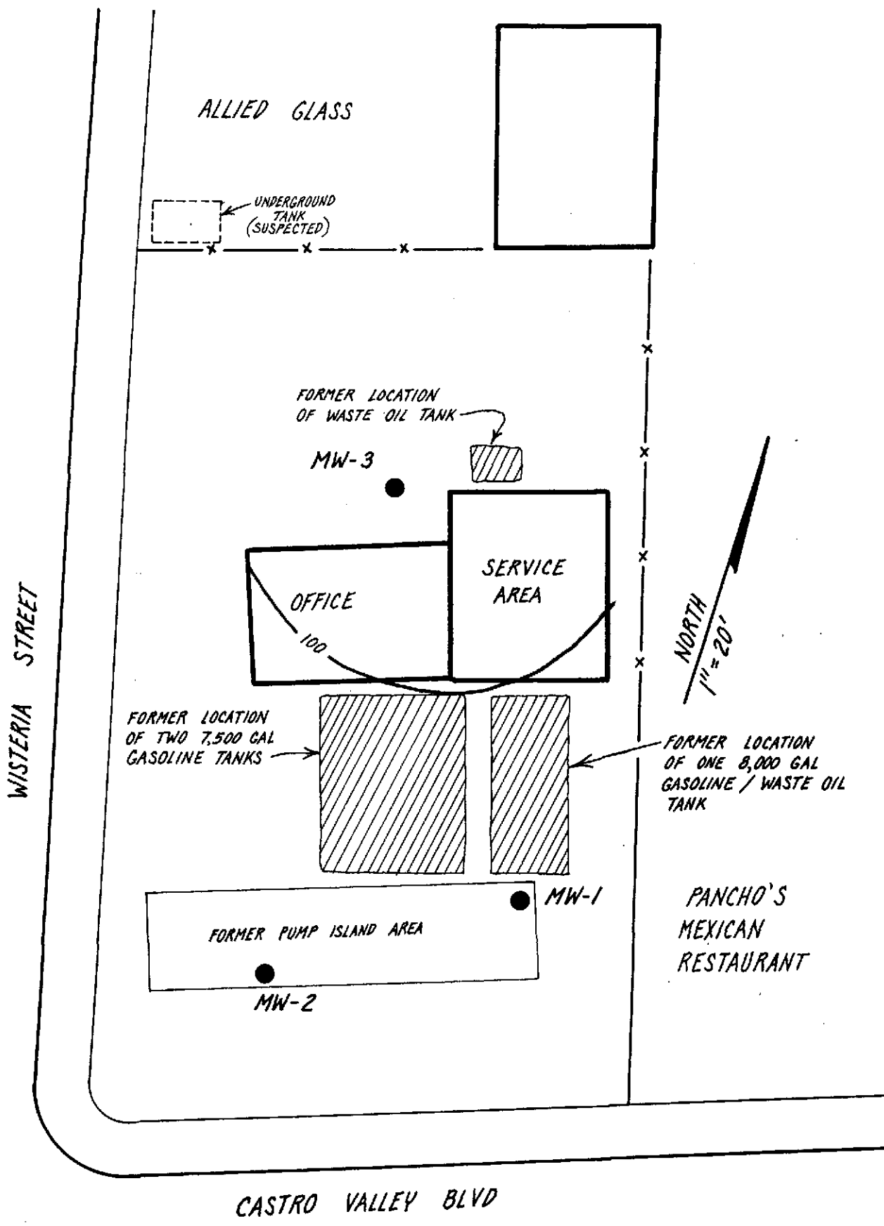
FIGURE 4. Lines of Equal Concentration of Gasoline in ug/L (ppb) in the Shallow Groundwater.
