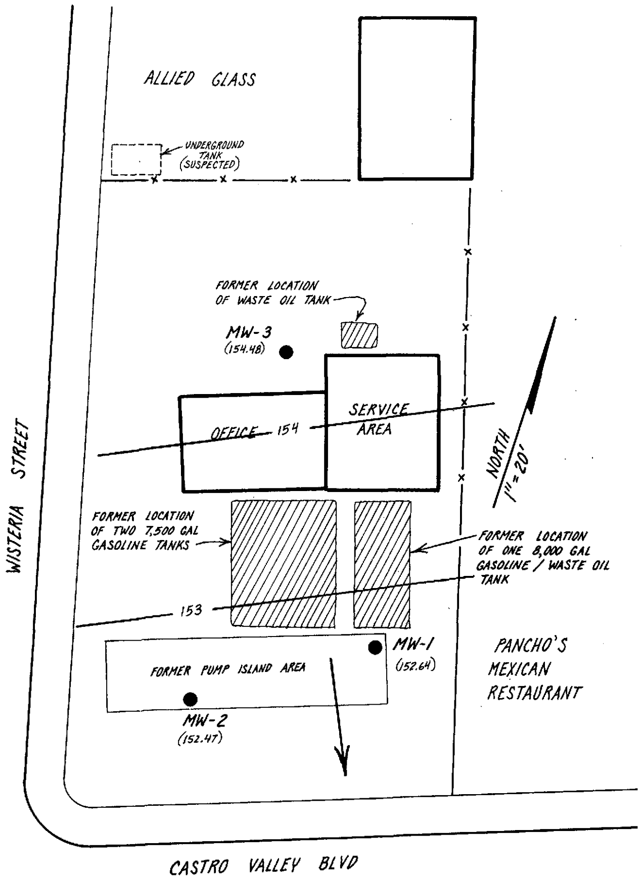
FIGURE 3. Shallow Water Table Contour Map (August 19, 1992).
