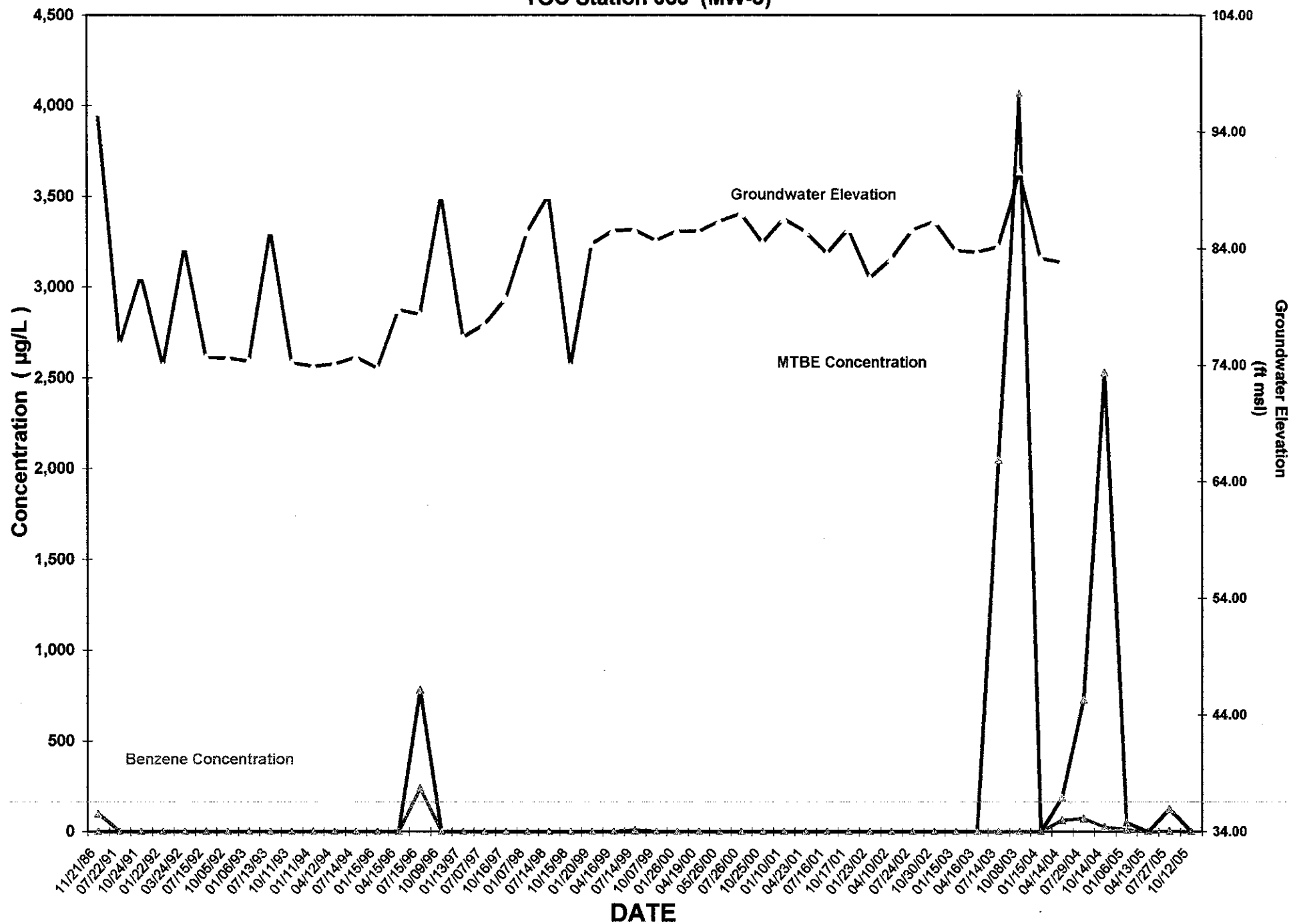
FIGURE 7C: Benzene / MTBE Concentrations and Groundwater Elevations vs. Time TOC Station 063 (MW-3)
