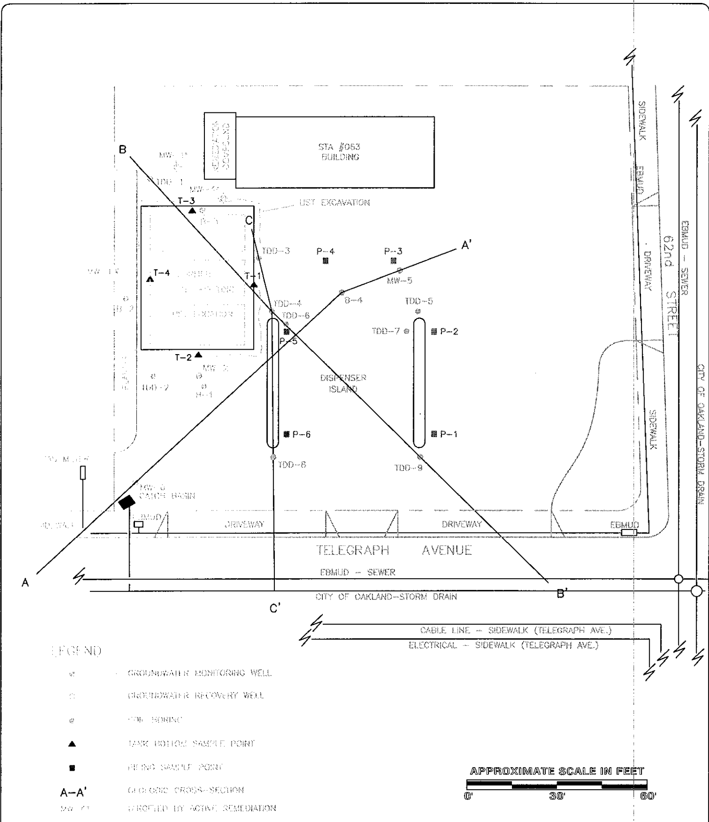
FIGURE 2 SITE PLAN WITH CONDUIT LOCATIONS THRIFTY SERVICE STATION #063 6125 Telegraph Avenue Oakland, CA
