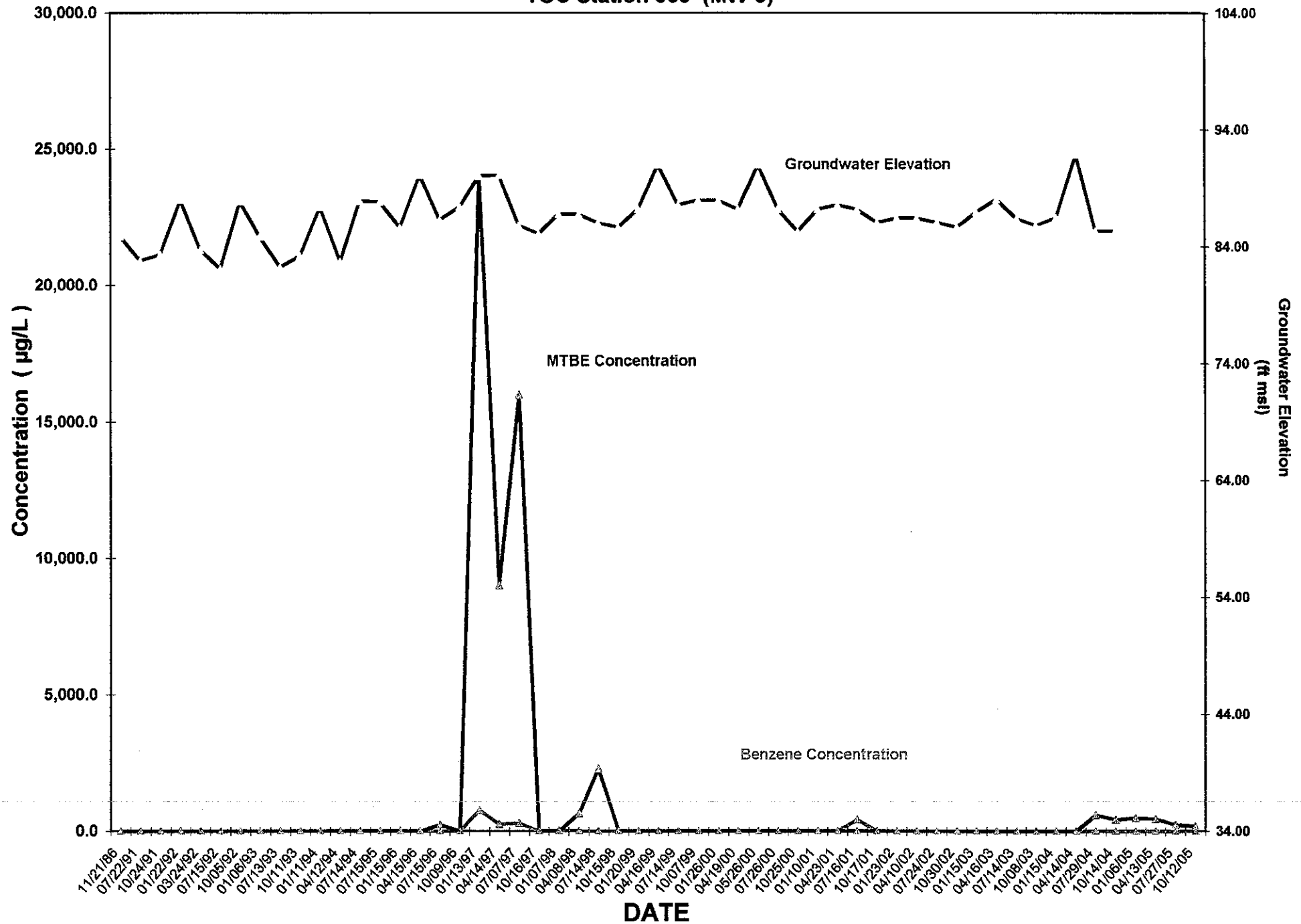
FIGURE 7E: Benzene / MTBE Concentrations and Groundwater Elevations vs. Time TOC Station 063 (MW-5)
