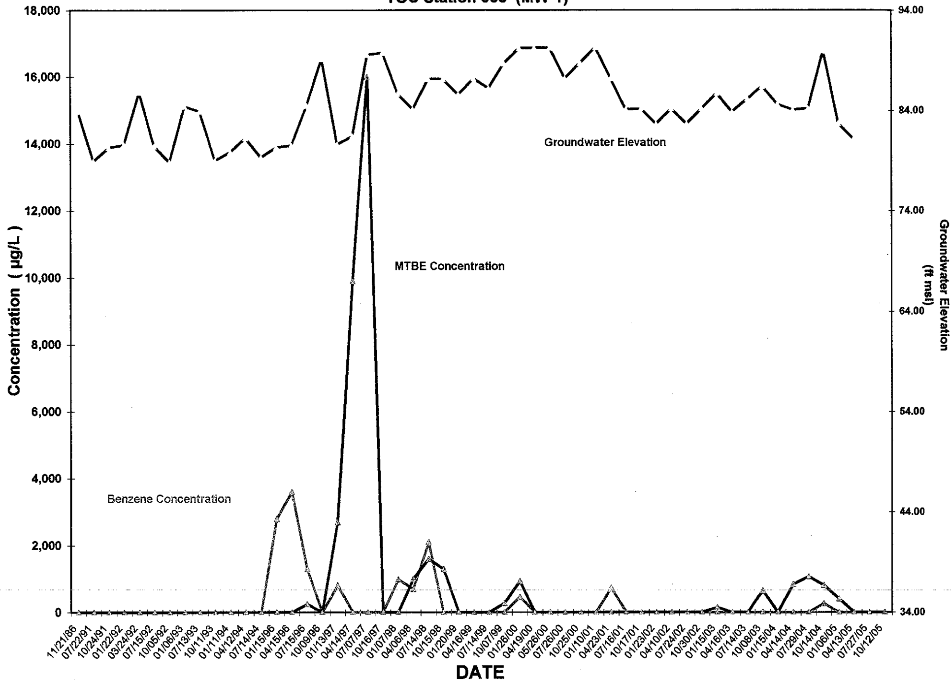
FIGURE 7A: Benzene / MTBE Concentrations and Groundwater Elevations vs. Time TOC Station 063 (MW-1)
