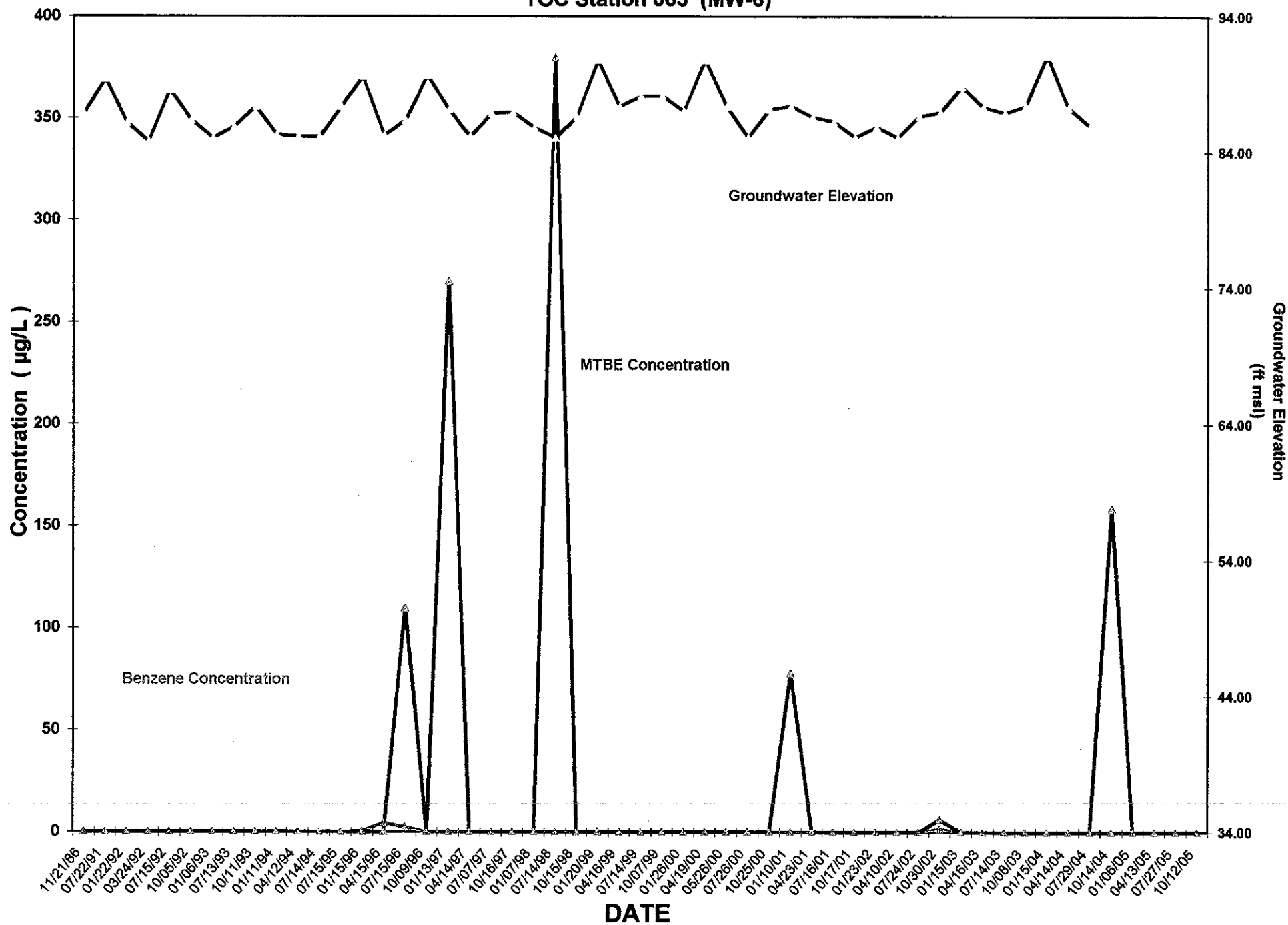
FIGURE 7F: Benzene / MTBE Concentrations and Groundwater Elevations vs. Time TOC Station 063 (MW-6)
