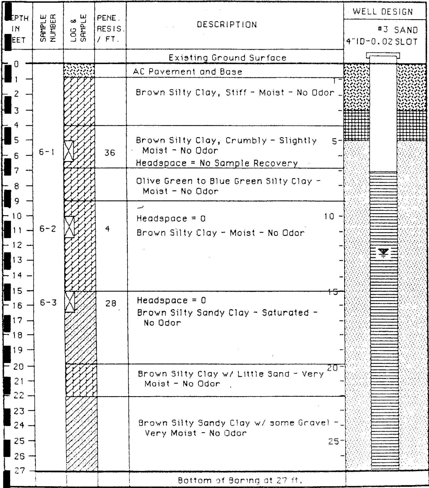
Figure 5 - Test Boring Log No. 5 - Monitoring Well No. MW-6
