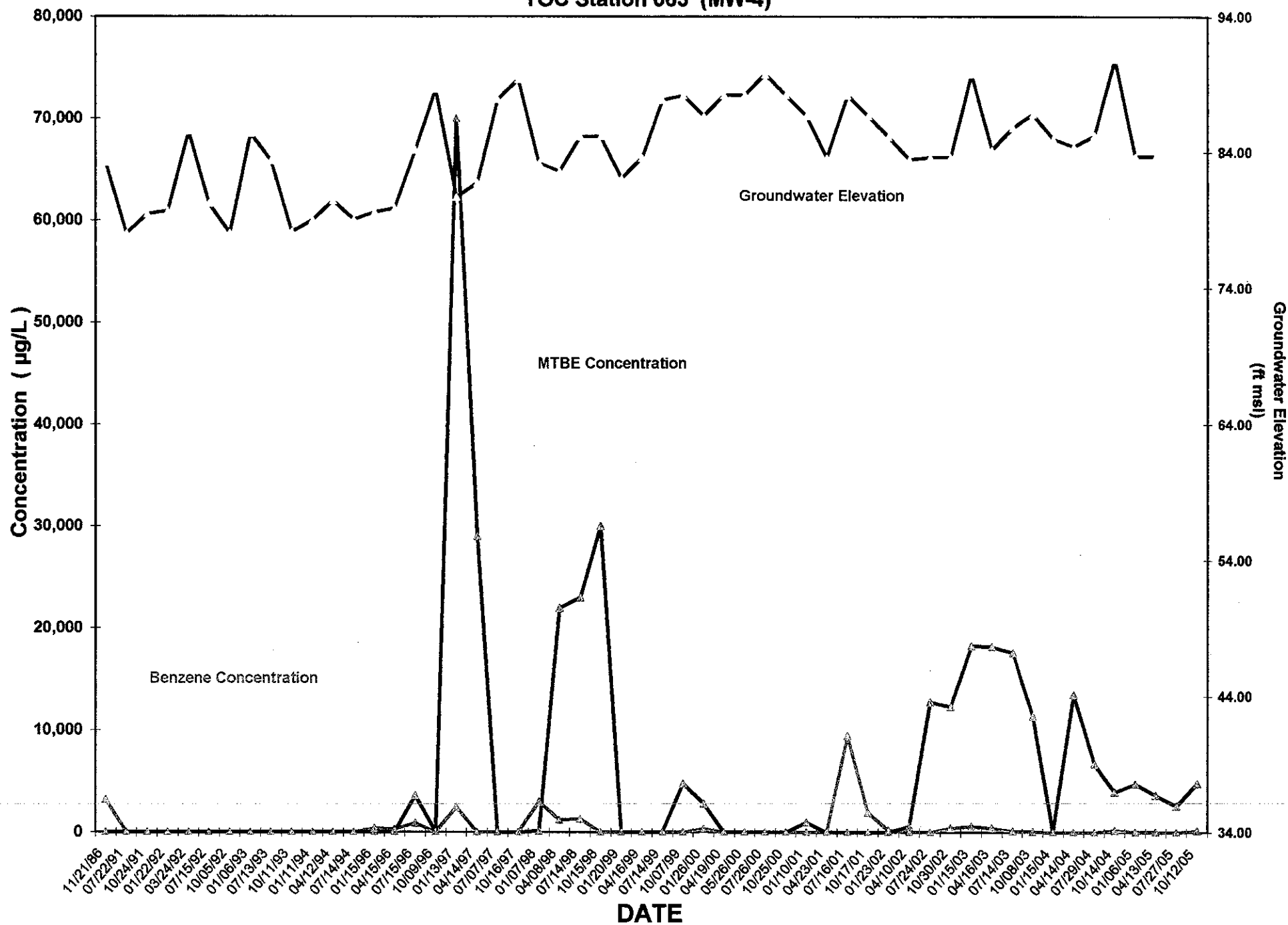
FIGURE 7D: Benzene / MTBE Concentrations and Groundwater Elevations vs. Time TOC Station 063 (MW-4)
