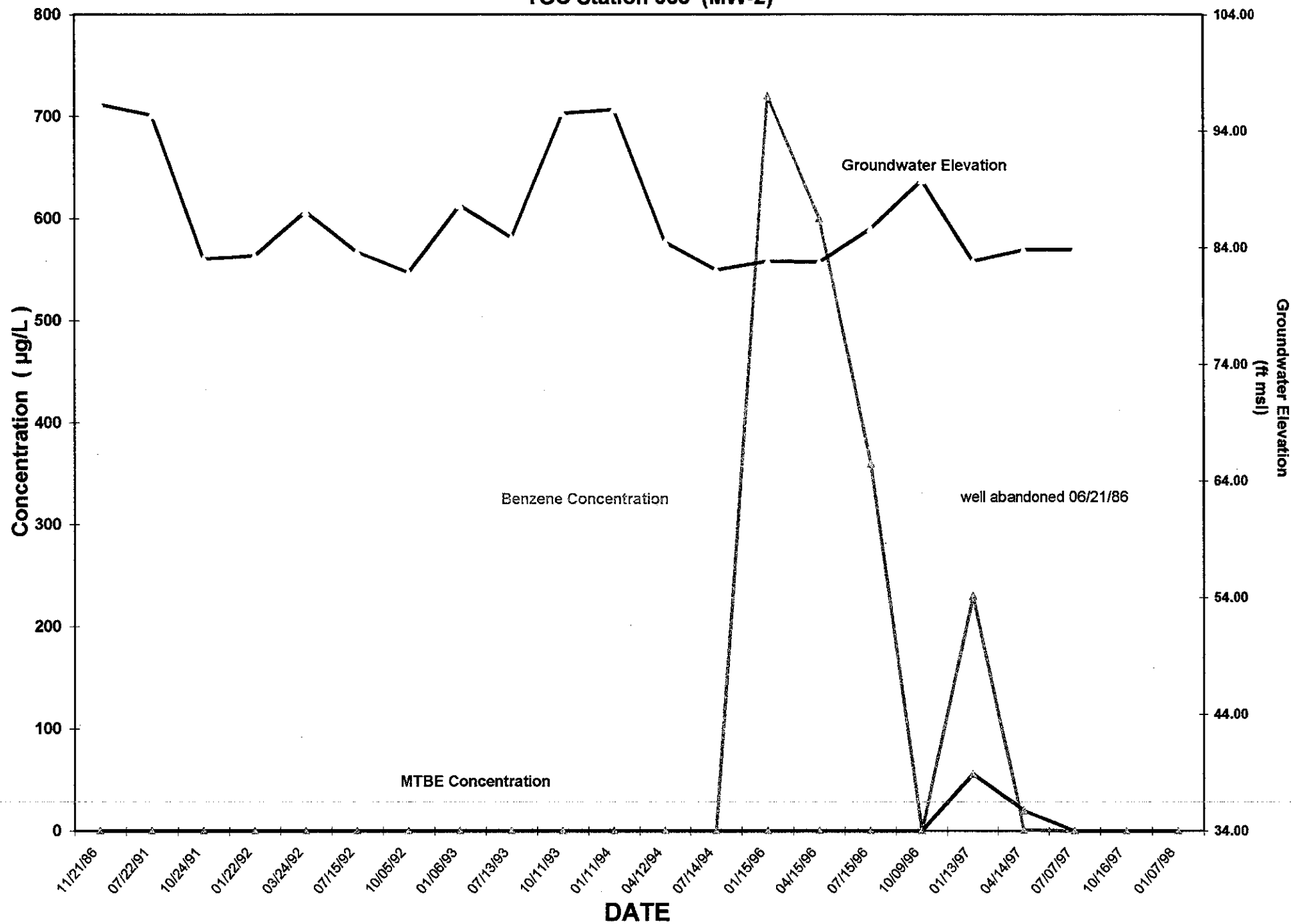
FIGURE 7B: Benzene / MTBE Concentrations and Groundwater Elevations vs. Time TOC Station 063 (MW-2)
