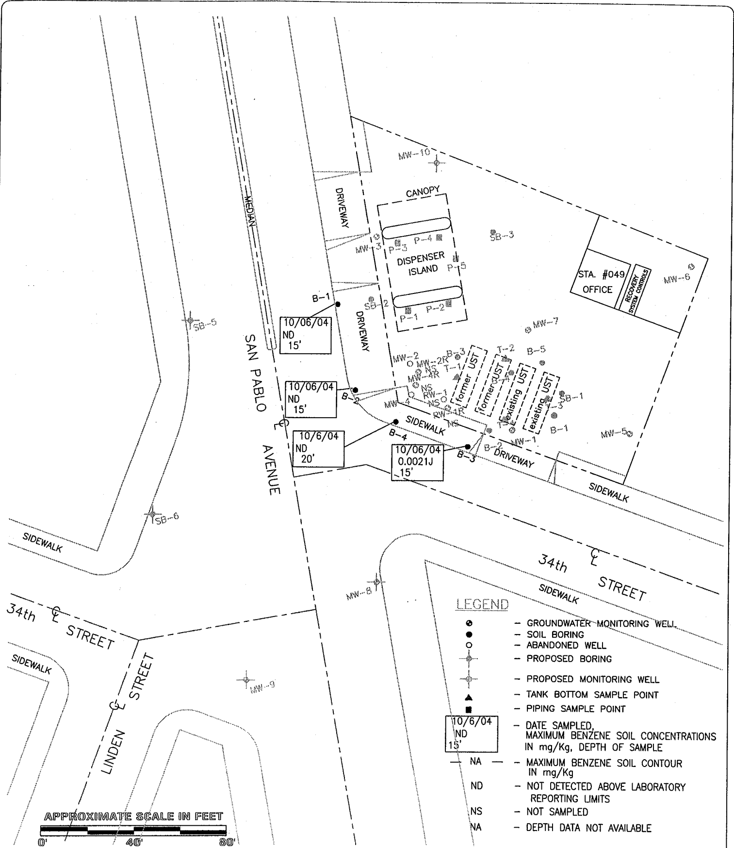
FIGURE 4K DISTRIBUTION OF BENZENE IN SOIL (Post-Remediation, 11-20 Feet Below Ground Surface) THRIFTY SERVICE STATION #049 3400 San Pablo Avenue Oakland, CA
