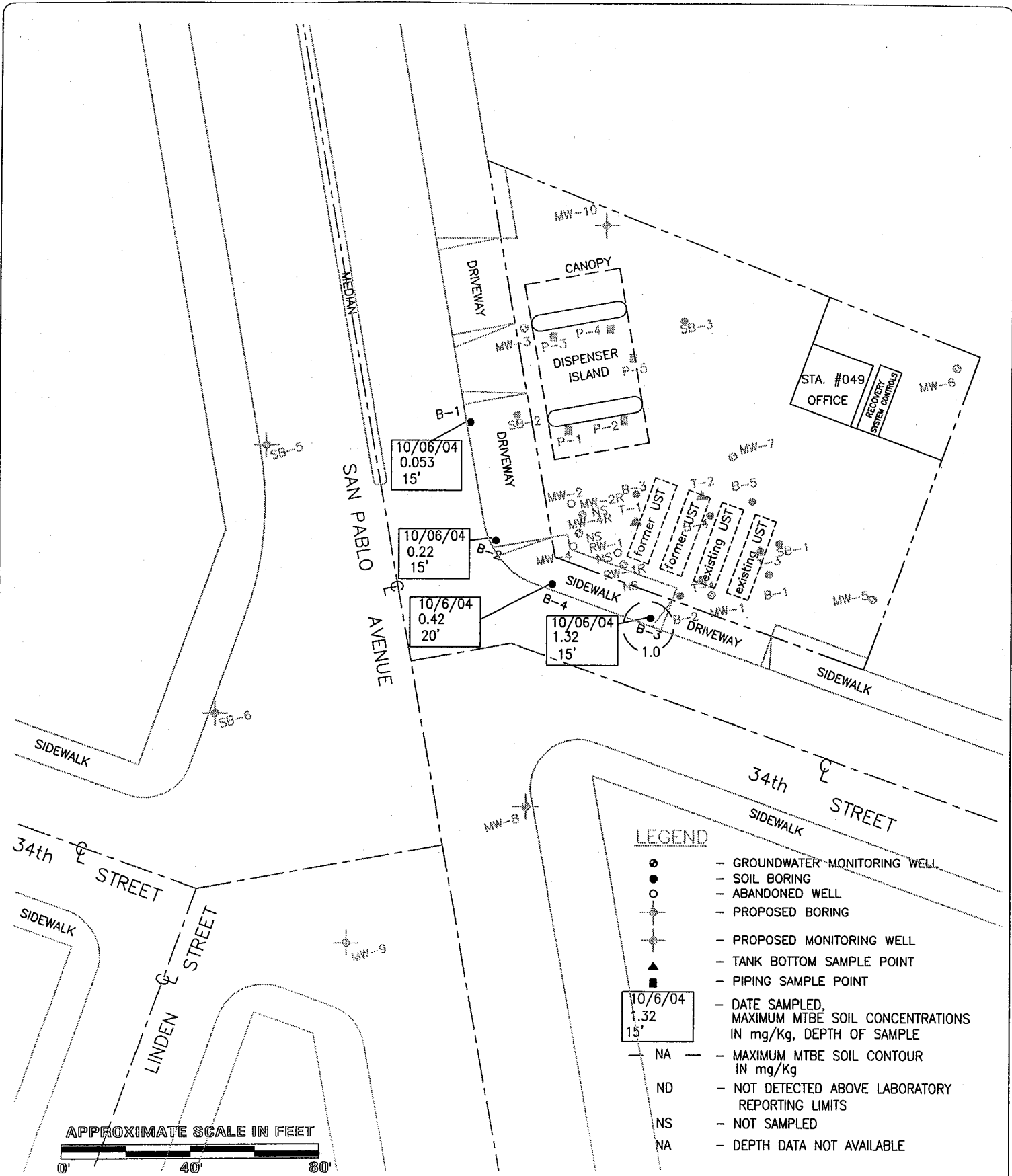
FIGURE 4L DISTRIBUTION OF MTBE IN SOIL (Post-Remediation, 11-20 Feet Below Ground Surface) THRIFTY SERVICE STATION #049 3400 San Pablo Avenue Oakland, CA
