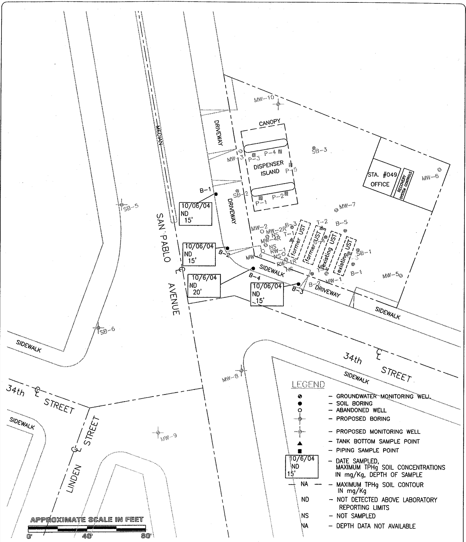
FIGURE 4J DISTRIBUTION OF TPHg IN SOIL (Post-Remediation, 11–20 Feet Below Ground Surface) THRIFTY SERVICE STATION #049 3400 San Pablo Avenue Oakland, CA
